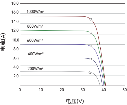
I-V曲线 (490W)
